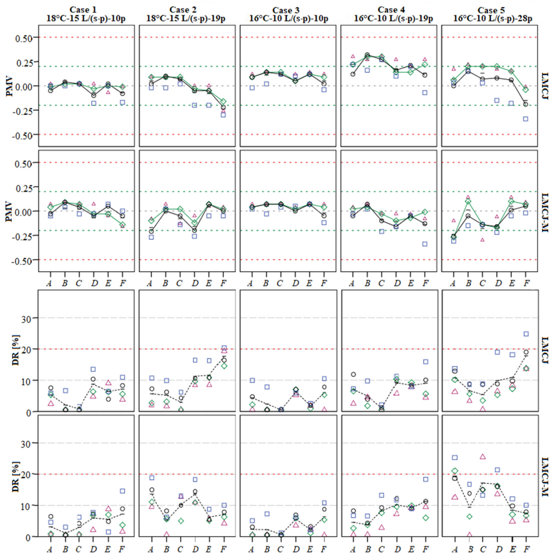
Figure 12. Thermal comfort (PMV and DR) at points A–F for LMCJ and LMCJ-M @ ■ = 0.1 m, ○ = 0.6 m, ◇ = 1.1 m, △ = 1.7 m, — = thermal Comfort for standing person, — = thermal comfort for seated person. - - - = limits for class B ISO-773, - - - = limits for class A ISO-7730, RH = 35%, CLO = 0.9, and MET = 1.1. Note: the lines/mean does not represent a gradient, it is only a comparison between points.
